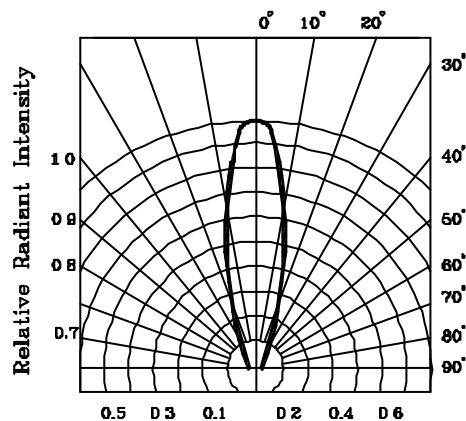
FIG.5 Radiant Diagram
