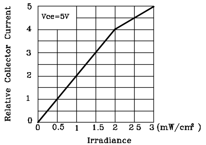
FIG.4 Relative Collector Current Vs. Irradiance
