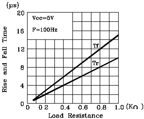
FIG.3 Rise And Fall Time Vs. Load Resistance
